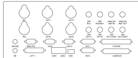
D 3 -CG Live Back Panel
